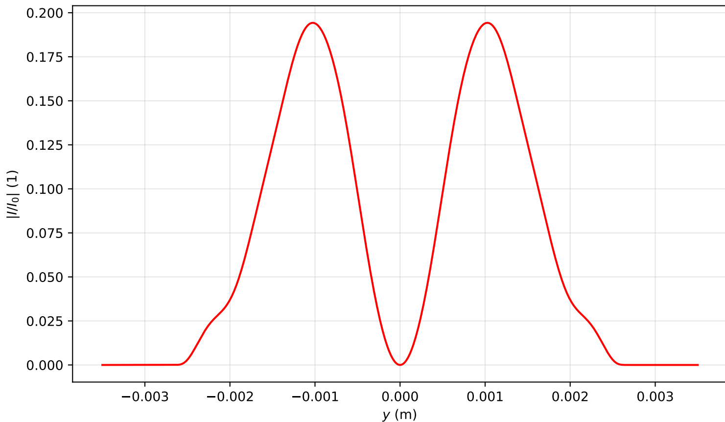
Intensity profile I(x=0, y, z=3.662)/I_0 , \text{Pin}=0.5\text{Pcr} , artificial time
